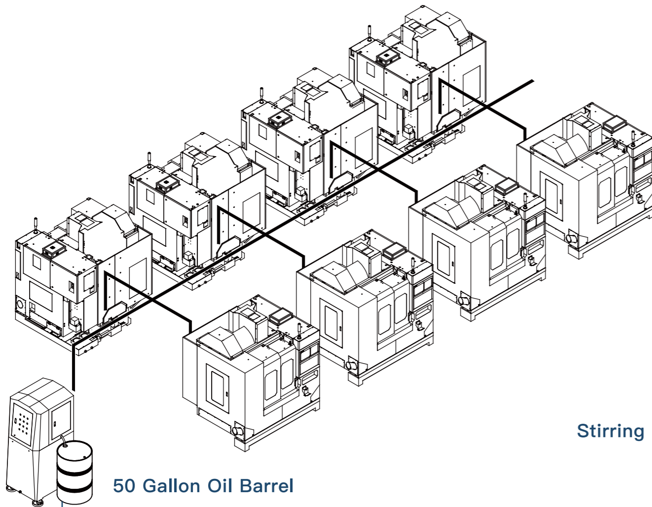
Auto Coolant Mixing Refill System
